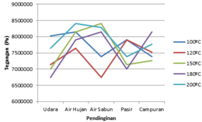
Figure 4.1 Graph Rated Voltage Vs Cooling
