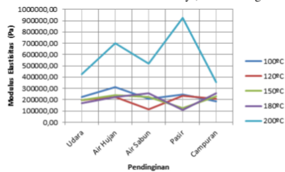
Figure 4.5 Modulus of Elasticity Vs Cooling
