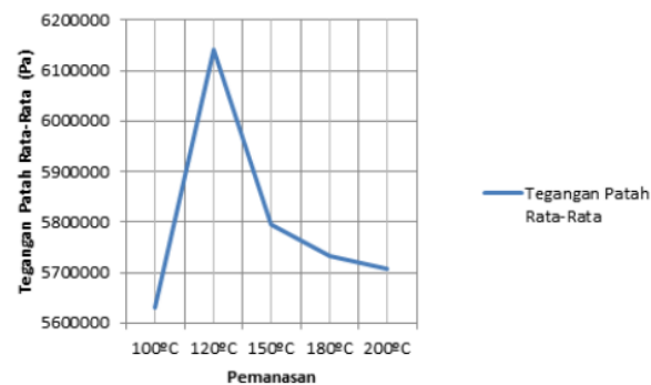
Figure 4.4 Graph Rated Voltage Broken Average Vs Temperature Heating
