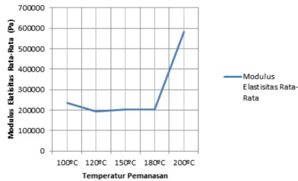
Figure 4.5. Modulus of Elasticity Average Vs Temperature Heating
