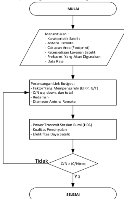
Figure 1. VSAT Network Planning Diagram
