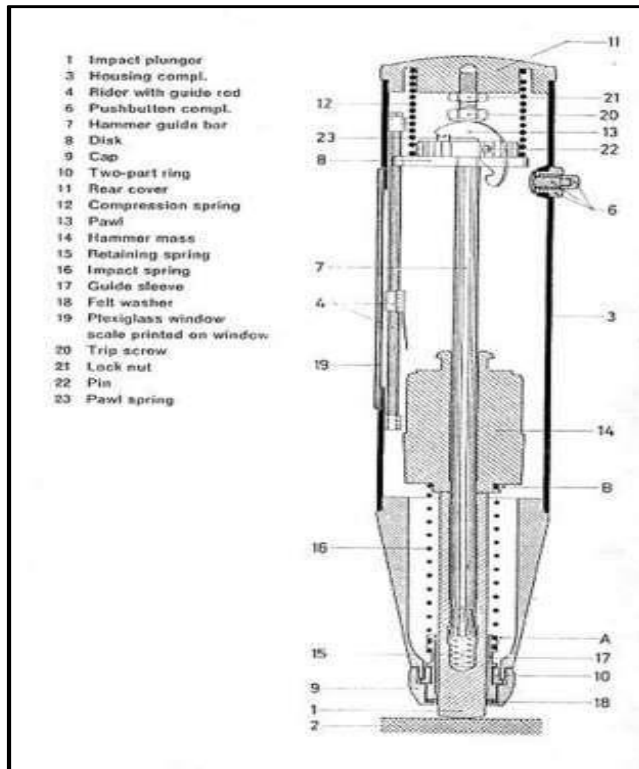
Gambar 3.7. Diagram Alat Hammer Test
