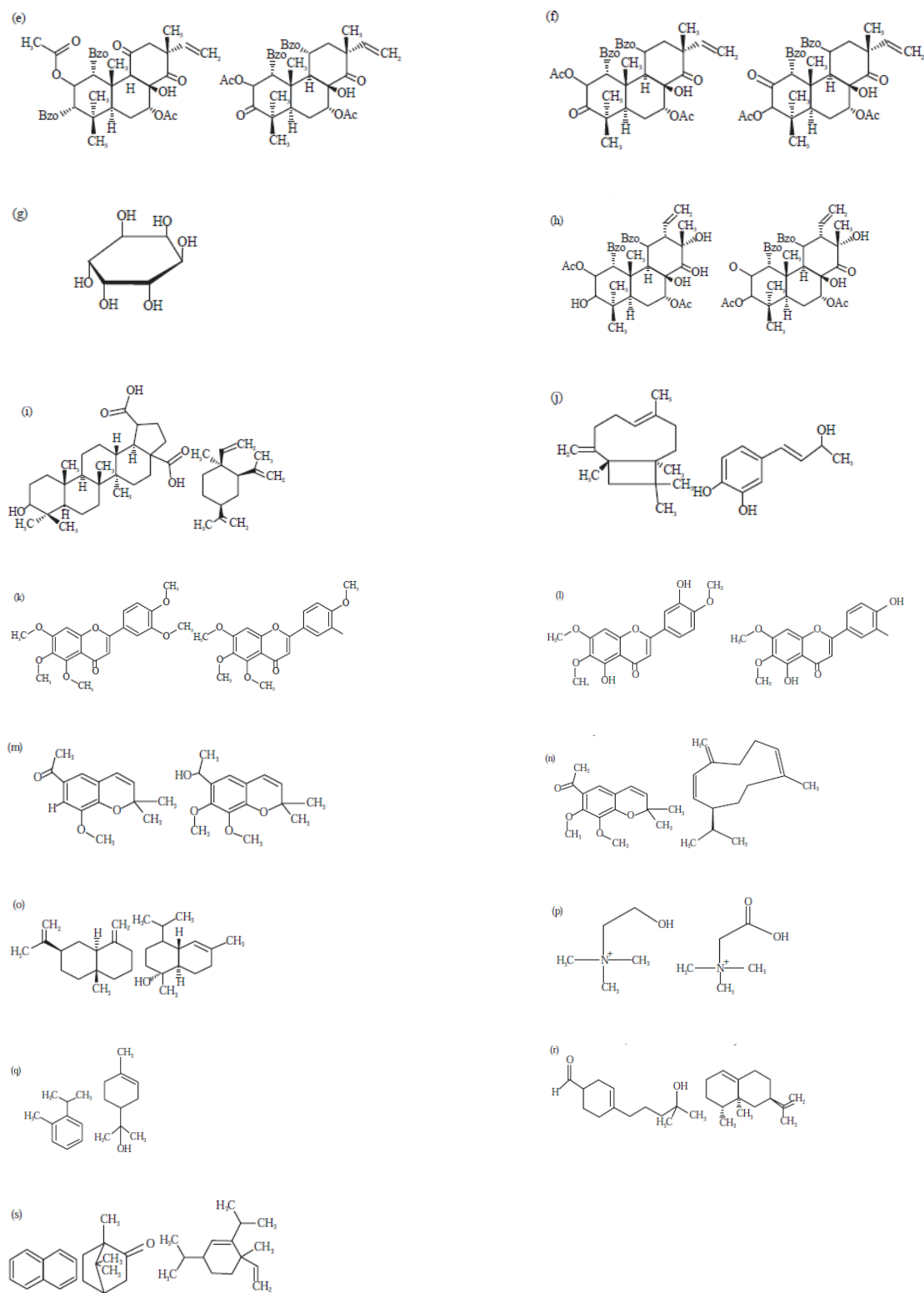
Figure 2. The chemical structure of typical and bioactive compounds isolated from Orthosiphon yaitu : (a) 3'-hydroxy-5,6,7,4'-tetramethoxyflavone neoorthosiphon A, (b) neoorthosiphon B \alpha -amyrin, (c) \beta -amyrin maslinic acid, (d) urosolic acid oleanolic acid, (e) orthosiphonone A orthosiphonone B, (f) orthosiphon A orthosiphon B, (g) myo-inositol, (h) neoorthosiphon A neoorthosiphon B, (i) betulinic acid \beta -elemene, (j) \beta -caryophyllene caffeic acid, (k) sinensetin tetra-methyl scutellarein, (l) eupatorin cirsimaritin, (m) acetovanillochromene orthochromene A, (n) methylripario chromene agermacrene-D, (o) \beta -selinen \alpha -cadinol, (p) choline betaine, (q) O-cyamenea-terpineol, (r) lyrol valencene, dan (s) naphthalin camphor \alpha -elemene (Singh et al 2015).
