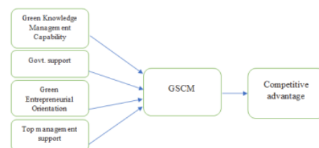
Figure 1. Theoretical framework
