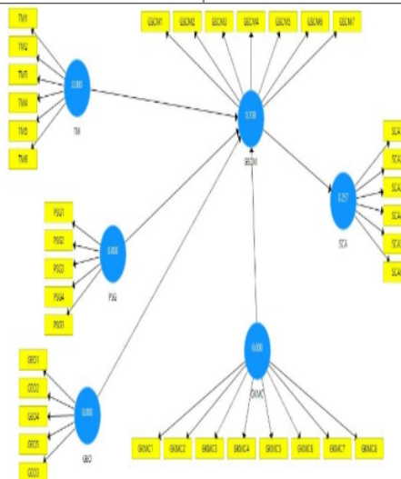
Figure 4. Blindfolding
