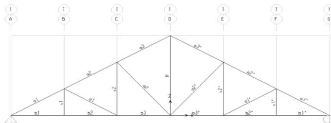
Figure 5. Modeling Wooden Framework by SAP 2000 [5],[7].
