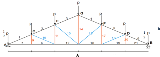
Figure 6. Modeling Wooden Framework by Joint of Method
