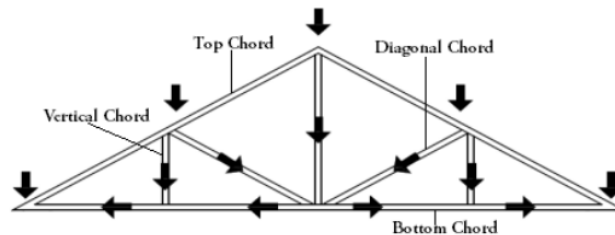
Figure 1. Wooden framework [4].
