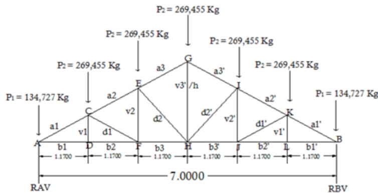
Figure 9. Design loading of wooden framework.
