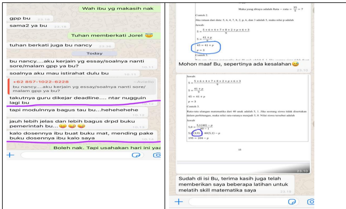
Figure 9. Student response to the statistics module
