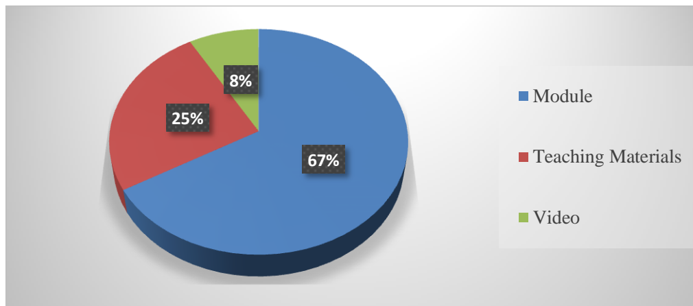
Pie Chart 1. Student Responses
