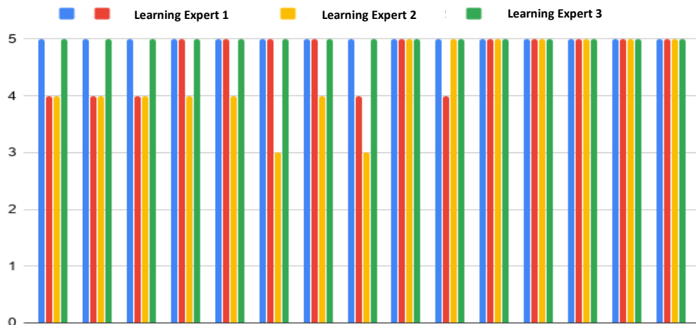
Figure 7. Learning Expert Validation
