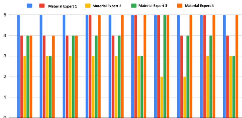
Figure 6. Statistical Material Expert Validation
