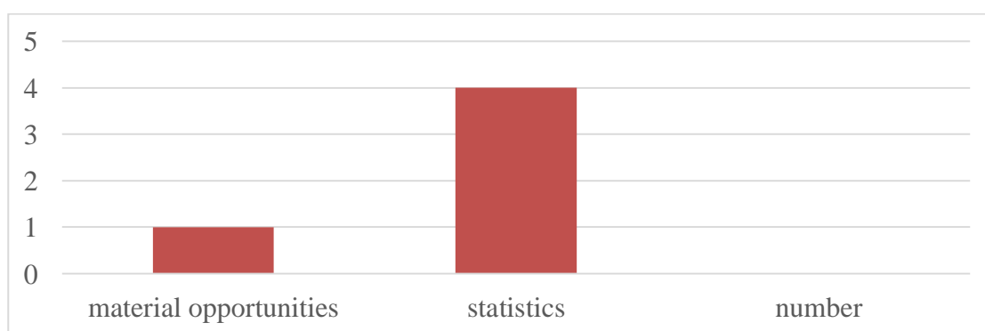
Bar Chart 1. Material is Difficult
