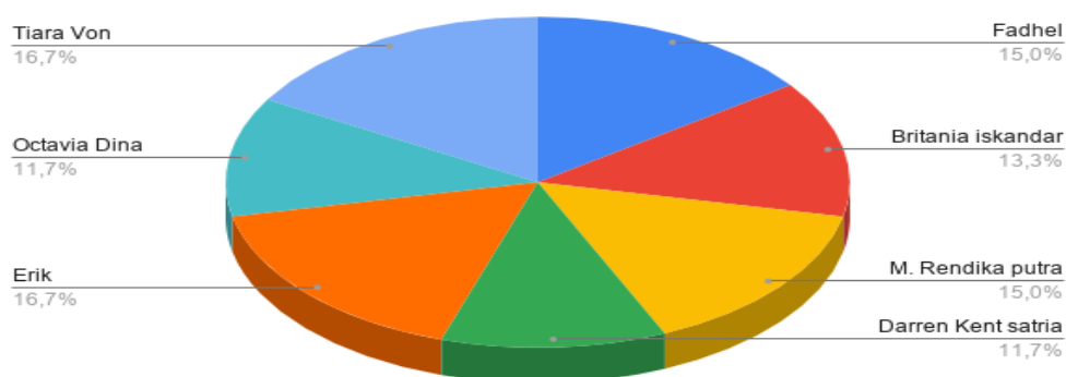
Figure 8. Small Scale Student Value Pie Chart
