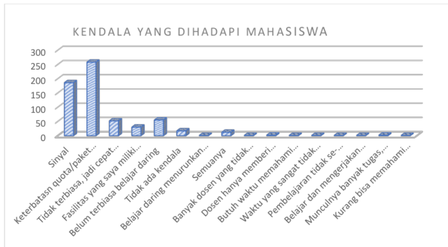
Graphic 1 , Constraints faced by Online Learning Respondents
