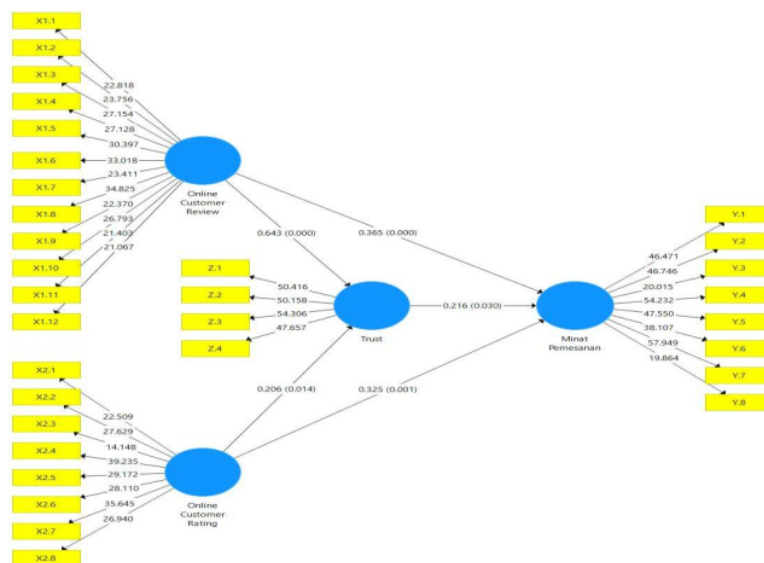
Figure 3 Inner Model
