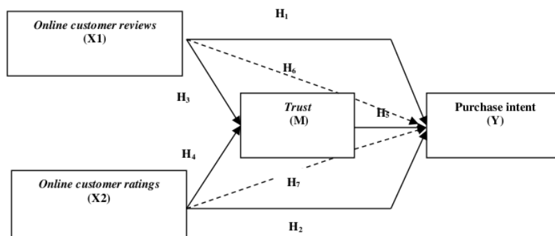
Figure 1 Path Diagram
