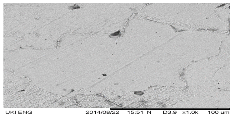
Figure 2. ST37 steel microstructure with magnification of 1000 times
