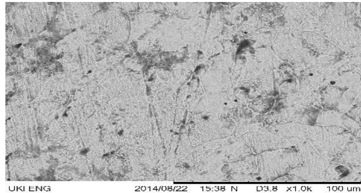
Figure 2. ST37 steel microstructure with magnification of 1000 times
