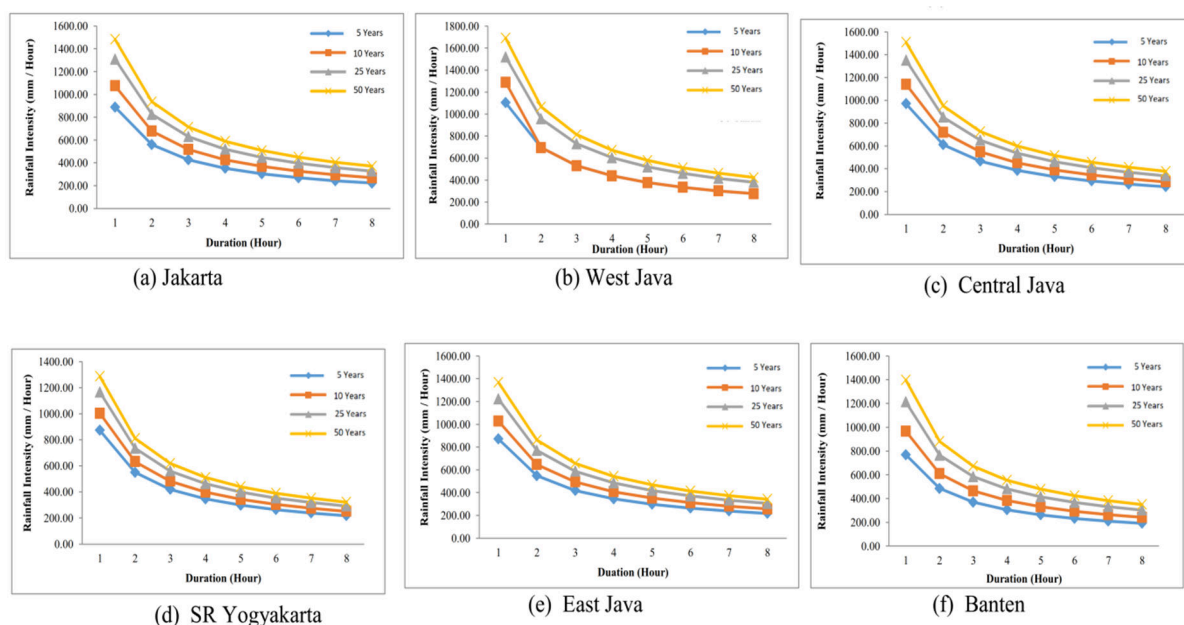
Figure 1. Intensity-Duration-Frequency (IDF) Curve
