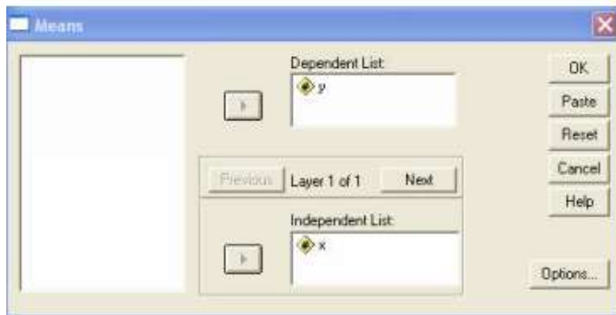
Gambar 8 Tampilan Kotak Dialog Means
