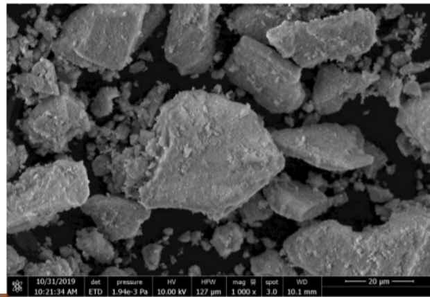
7 Figure 5. The results of SEM HA with a magnification of 1000x.
