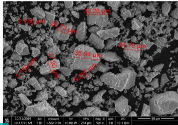
16 Figure 4. The results of SEM HA with a magnification of 500x.
