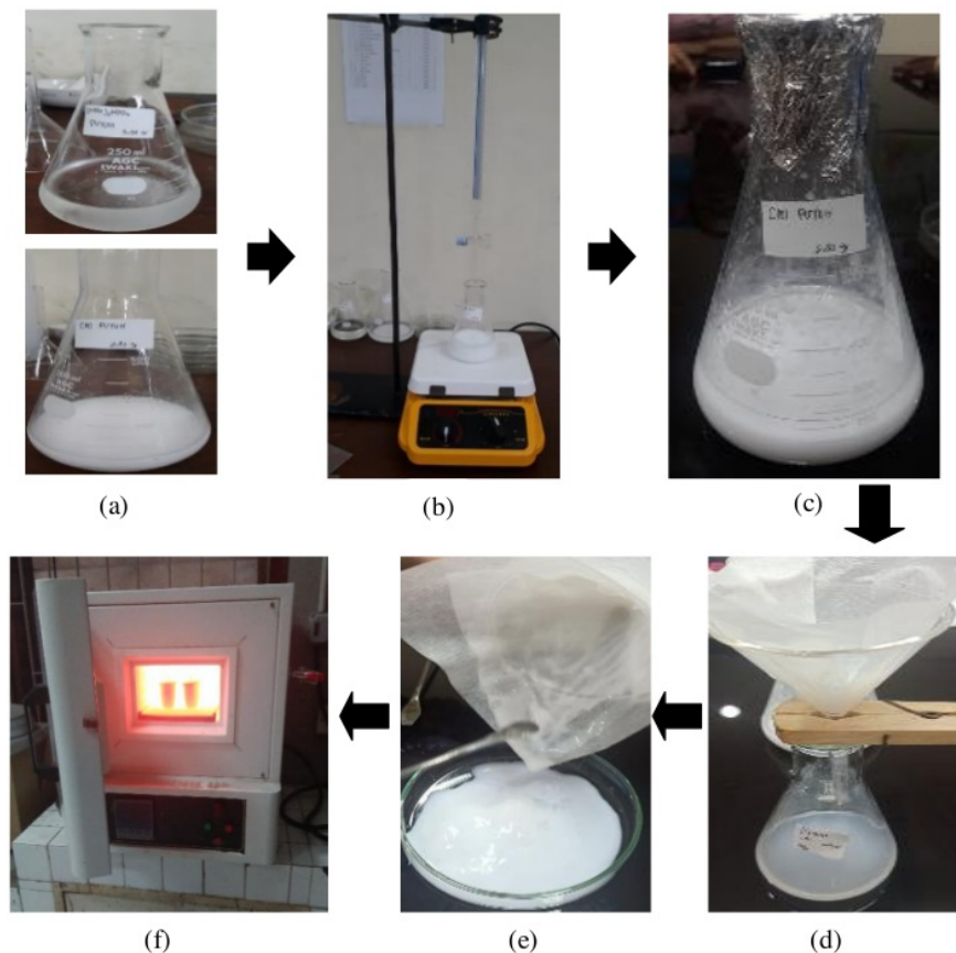
Figure 2. HA synthesis process (a) CaO and (\text{NH}_4)_2\text{HPO}_4 solutions (b) CaO drops (\text{NH}_4)_2\text{HPO}_4 (c) Precipitated one night (d) Washed and filtered (e) Oven dried (f) Sintering for 5 hours.
