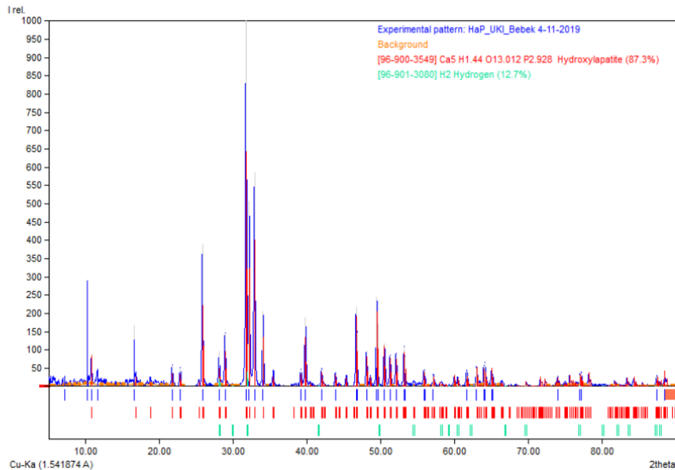
Figure 3. The XRD diffraction pattern of duck eggshells resulted from sintering at 900 °C for 5 hours.
