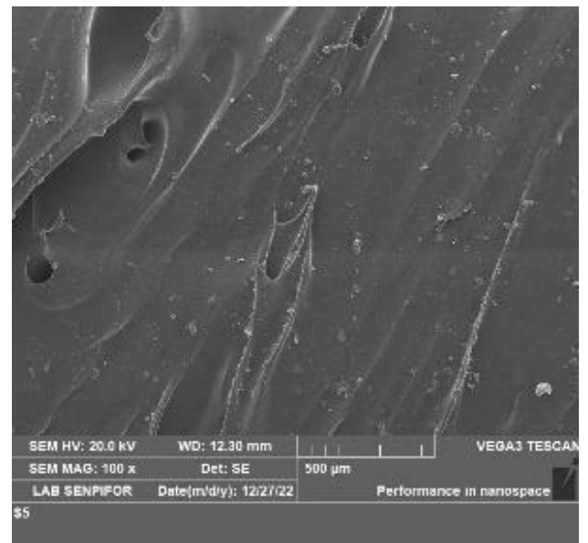
Fig. 10. SEM results of microstructure for specimen B-10 at 100x magnification.
