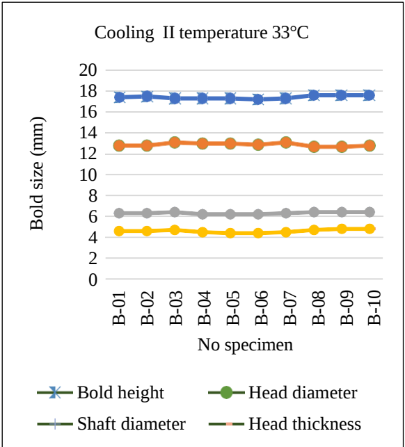
Fig. 4. Cooling graph of specimens at 33°C.
