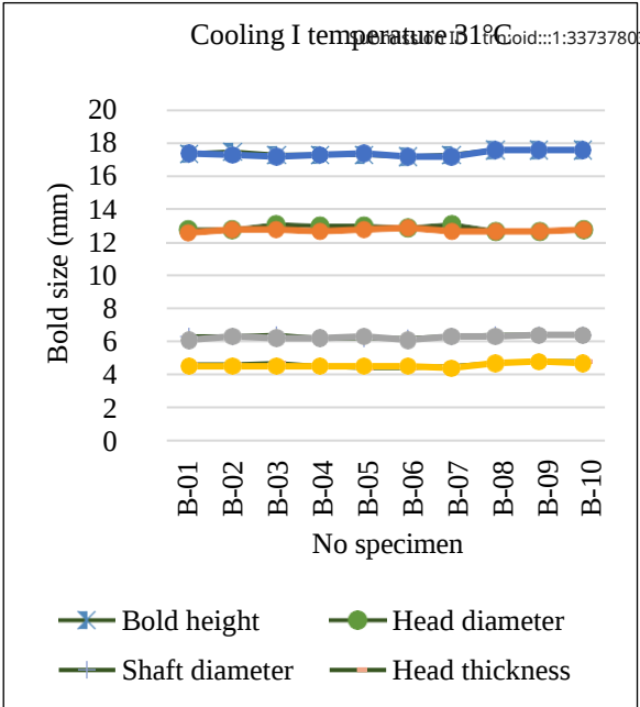
Fig. 3. Cooling graph of specimens at 31°C.
