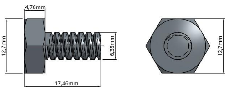
Fig. 1. Printed specimen.
