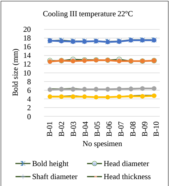
Fig. 5. Cooling graph of specimens at 22°C.
