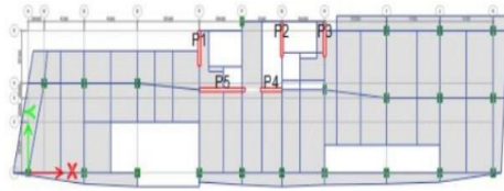
Gambar 1. Denah Shear wall Eksisting
