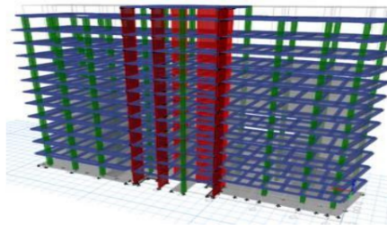
Gambar 2. Pemodelan 3D Shear wall Eksisting
