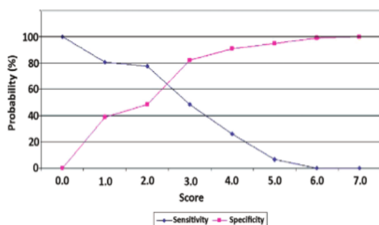
Figure 1 - Sensitivity and specificity curves. Sensitivity and specificity curves were used to determine the optimal cut-off value. There were 2 alternative points of intersection: a score of 2 (sensitivity 77.4%, specificity 48.4%) and a score of 3 (48.4% sensitivity, 82.3% specificity).
