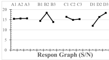
Figure 4. Response graph (S/N) max power
