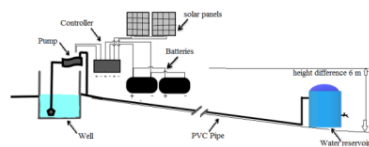
Figure 1. Water distribution scheme
