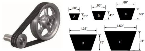
Figure 1. Belts and belt type selection
