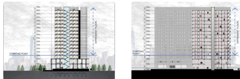
Figure 4. Experiment floors and starting point of measurements.
