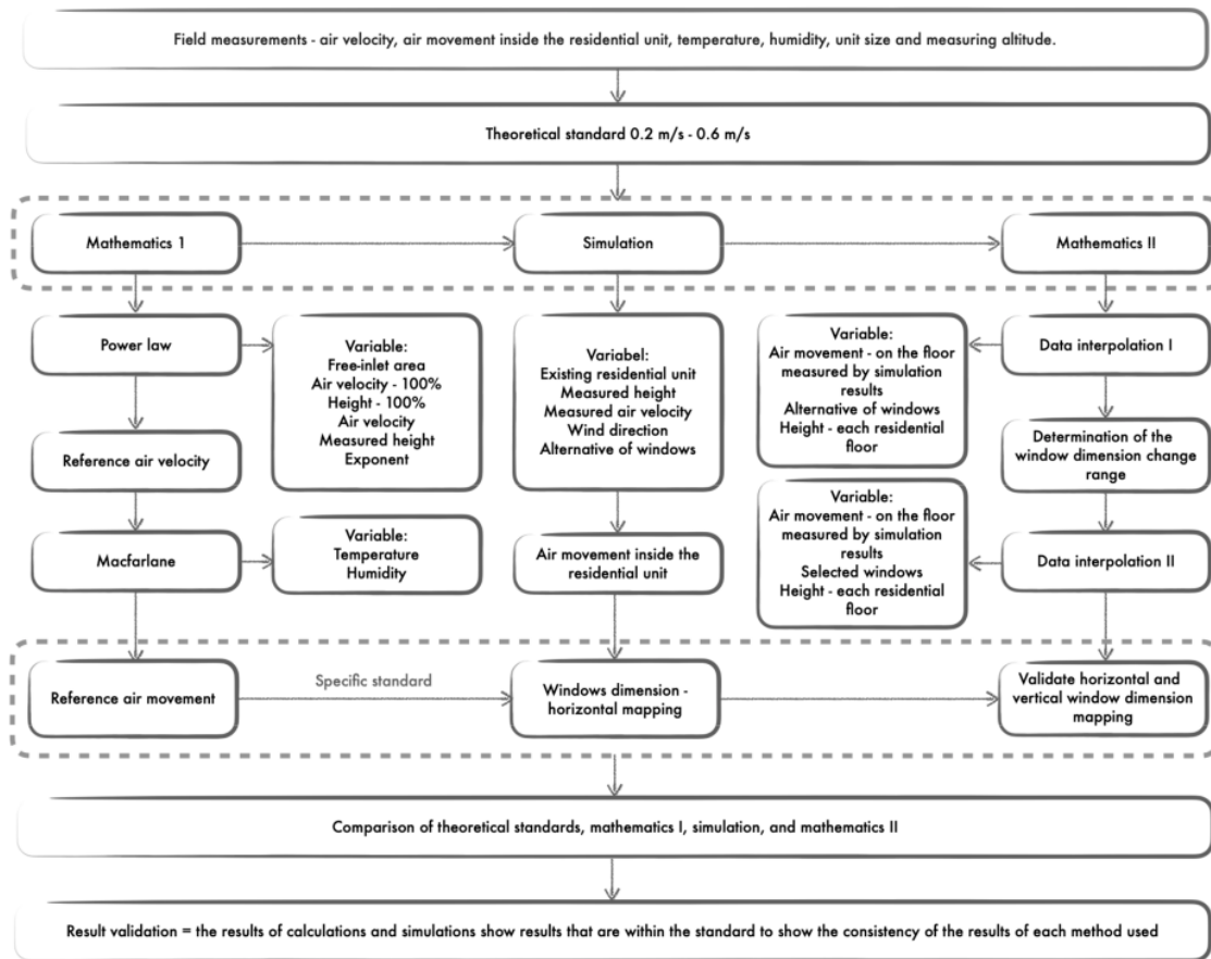
Figure 7. Research workflow.
