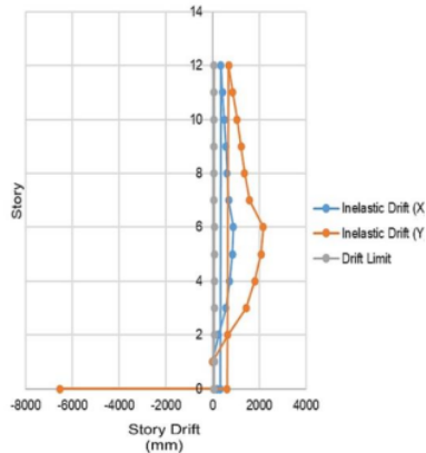
Figure 6. Story drift of earthquake loads response spectrum
