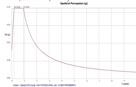
Figure 2. Response spectrum MRT Hub Dukuh Atas Jakarta
