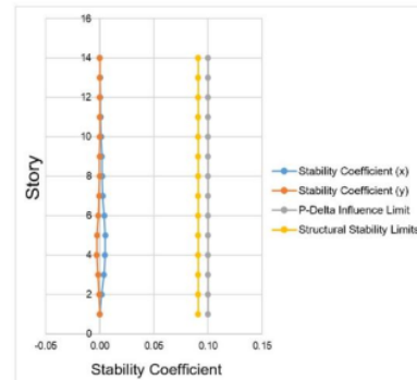
Figure 13. Stability against influence P-Delta EI centro 1940 earthquake
