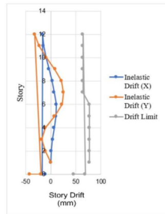
Figure 8. Story drift of earthquake loads ChiChi Taiwan
