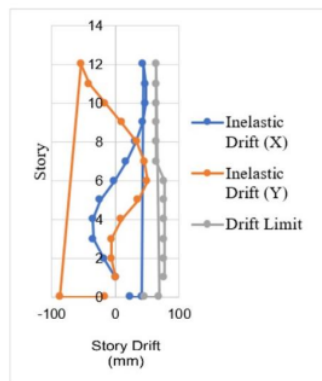
Figure 7. Story drift of earthquake loads Kobe University, Japan
