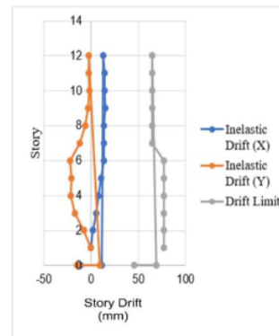
Figure 9. Story drift of earthquake loads EI centro 1940
