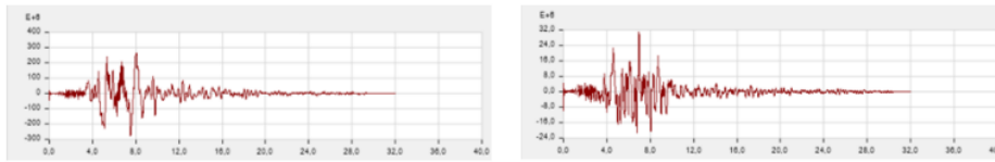
Gambar 3. Grafik Acceleration Gempa Kobe, Kanan (X), Kiri (Y)
