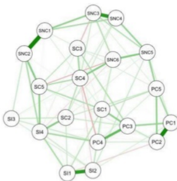
1 Figure 3. A Network Model interaction between the factor structure of Internet addiction.
