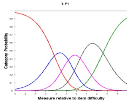
1 Figure 2. Category Probability
