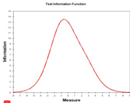
1 Figure 1. Test Information Function (TIF)
