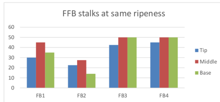
Figure 13. The hardness of 4 samples of FFB stalks.
