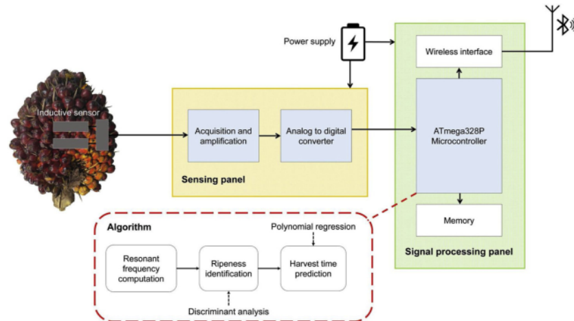
Fig. 2. Inductive sensor system architecture.
