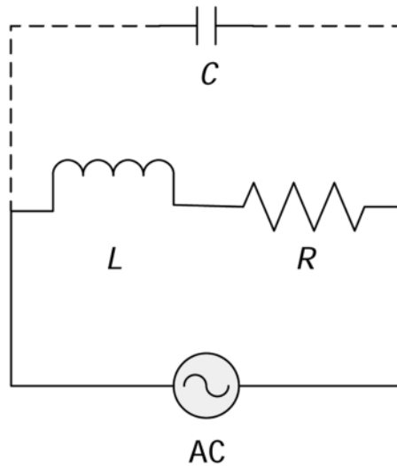
Fig. 3. RLC circuit in an inductive sensor system.
