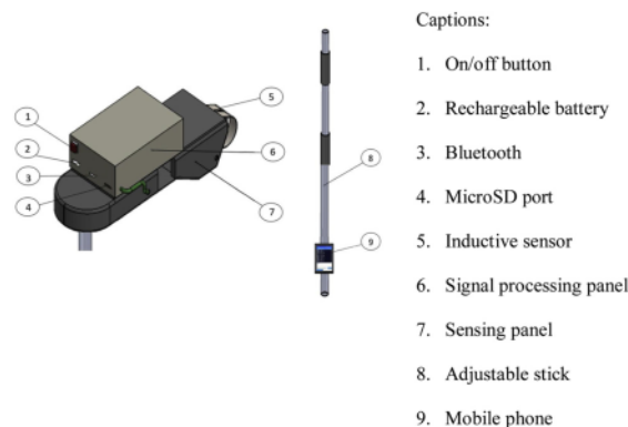
Fig. 1. Inductive sensor system.
