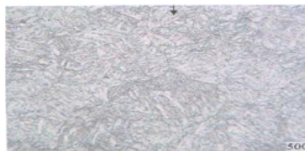
Figure 6. Micrograph basic material in the form of ferrite (white) and pearlite (black). E7016
