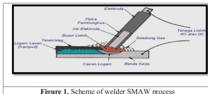
Figure 1. Scheme of welder SMAW process
