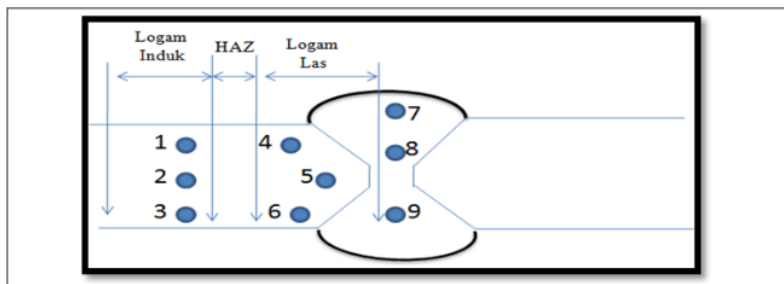
Figure 3. Investigation point of specimen type CS32 steel
