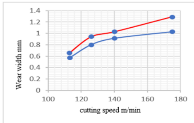
Figure 4. Wear width comparison graph.
