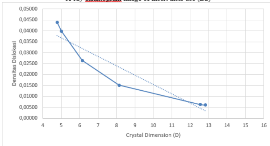
Figure 9. Relationship of crystal size to dislocation density of insert after use (B1).
