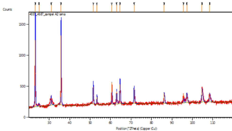
X-ray difraktogram image of insert after use (B2)
