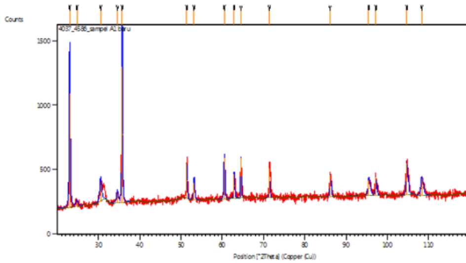
X-ray Difaktogram image of insert (B1)
