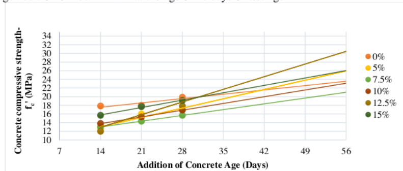
FIGURE 7. Compression strength prediction in 56-days concrete
