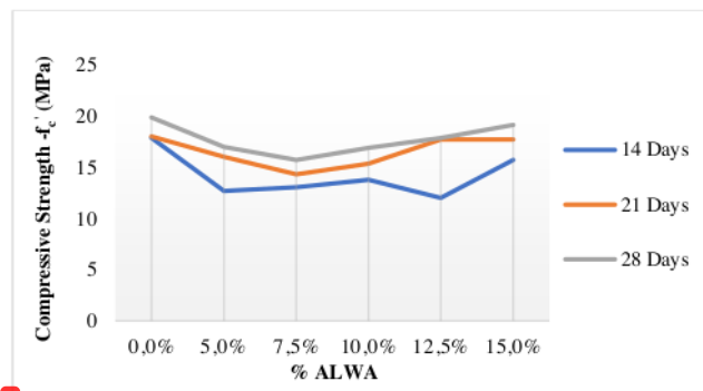
FIGURE 5. Compressive strength of 12.5% fly ash mixed concrete with a variation of ALWA addition
