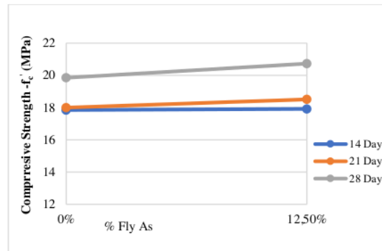
FIGURE 4. Compressive strength of fly ash mixture
