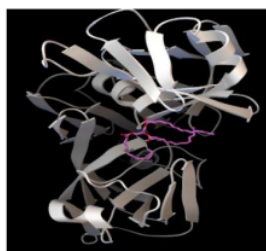
Figure 2: Pose Ligand Trimyristin and Plasmepsin receptor
