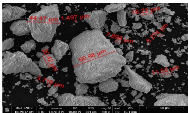
Fig. 2. SEM HA results with 500x magnification
