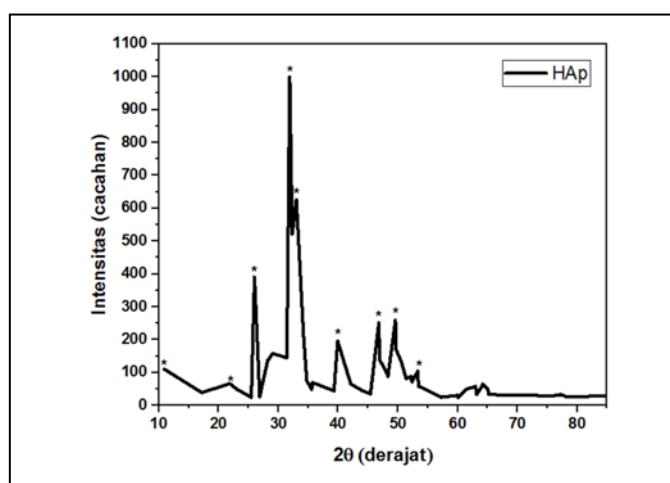
Fig. 1. XRD HA diffraction pattern from quail eggshell
