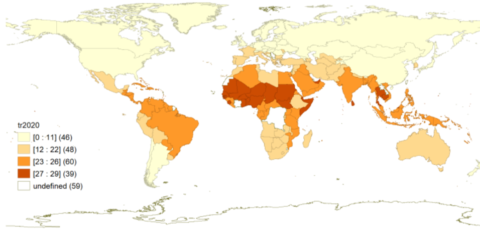
Figure 1. Spatial Patterns of Temperature in 2020
