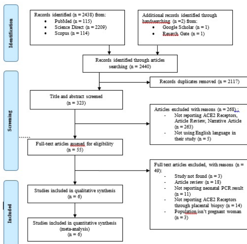
Figure 1 PRISMA Flowchart
